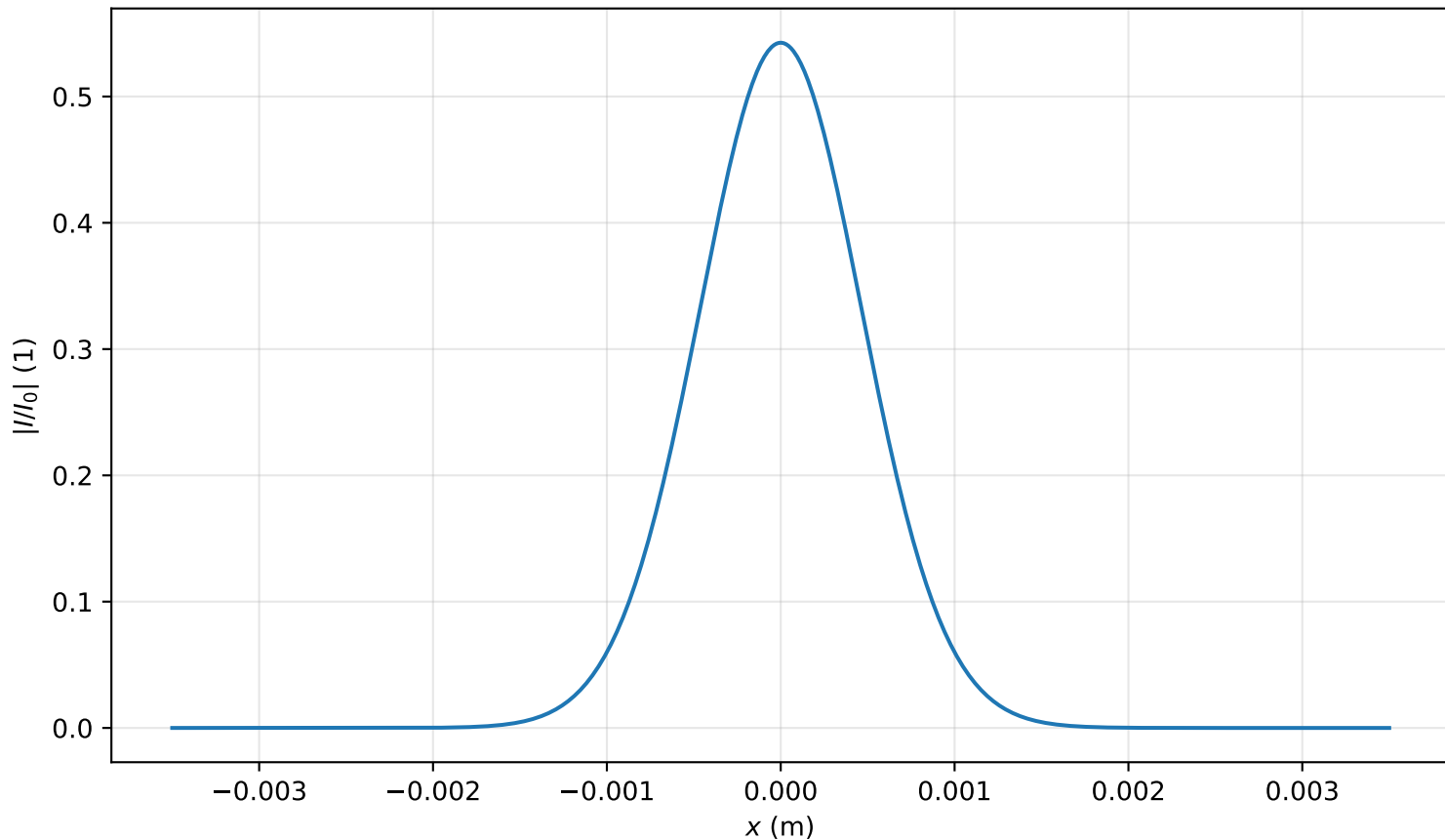
Intensity profile I(x, y = 0, z = 1.990m)/I_0 , P_{in}=0.1P_{cr} , artificial time
